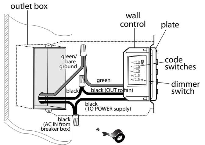
(wiring for wall control)
